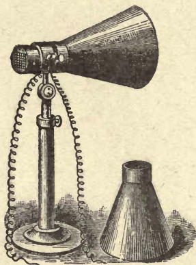
FIG. 6.—Thermo-pile.
