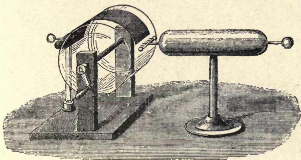
FIG. 5.—Frictional electrical machine.
